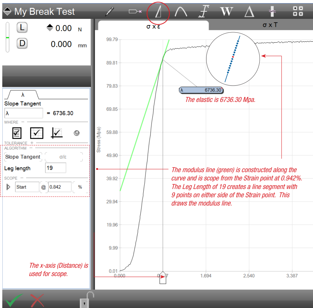
Tangent Slope Shows elastic at tangent point
