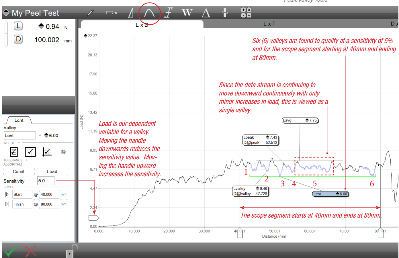
Peel test using Peak/Valley Measurement Shows the number of Valleys (Count) for the scope segment and a sensitivity of 5%
