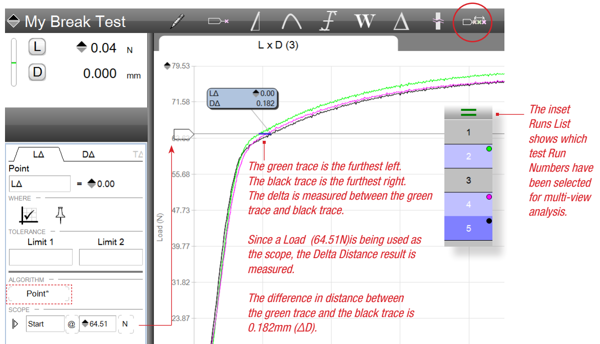
Multi-Run Graph View Finding Delta Distance between all selected Runs
