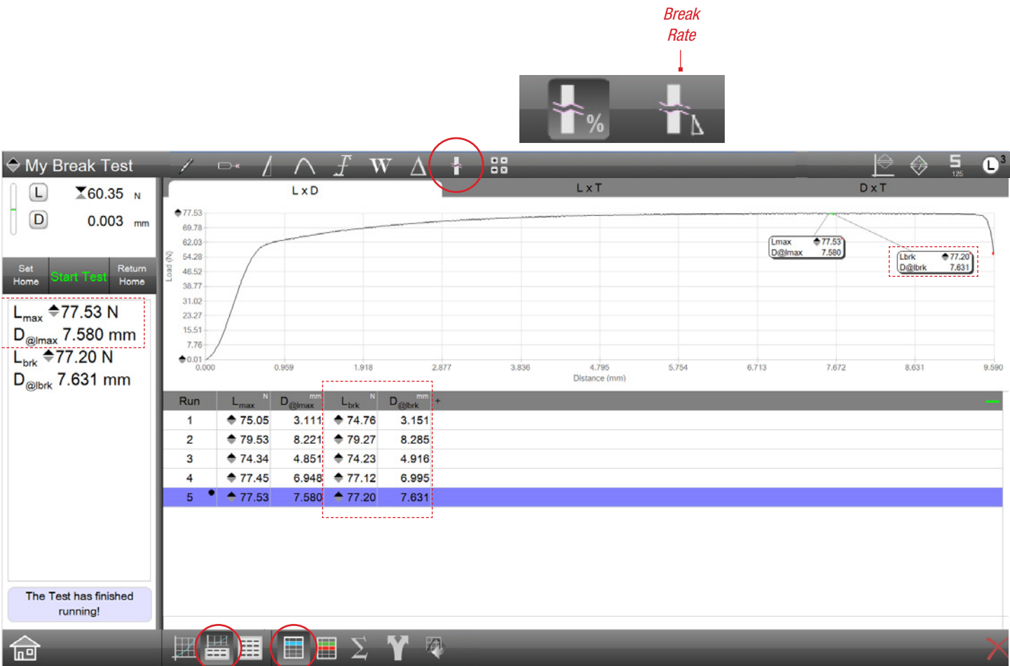
Split Graph - Data View Finding Break load using a Rate (N/mm) in load after Lmax
