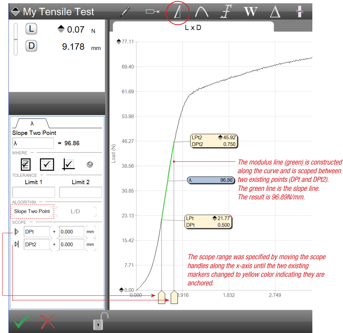
Two-Point Slope Shows elastic using two anchor points
